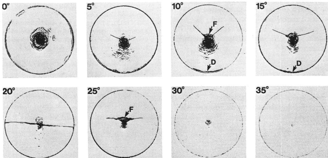
Figure 2 Typical damage produced by 620 \text{ m sec}^{-1} impacts at various angles (marked). The impact is from top (“upstream” direction) to bottom (“downstream” direction).
